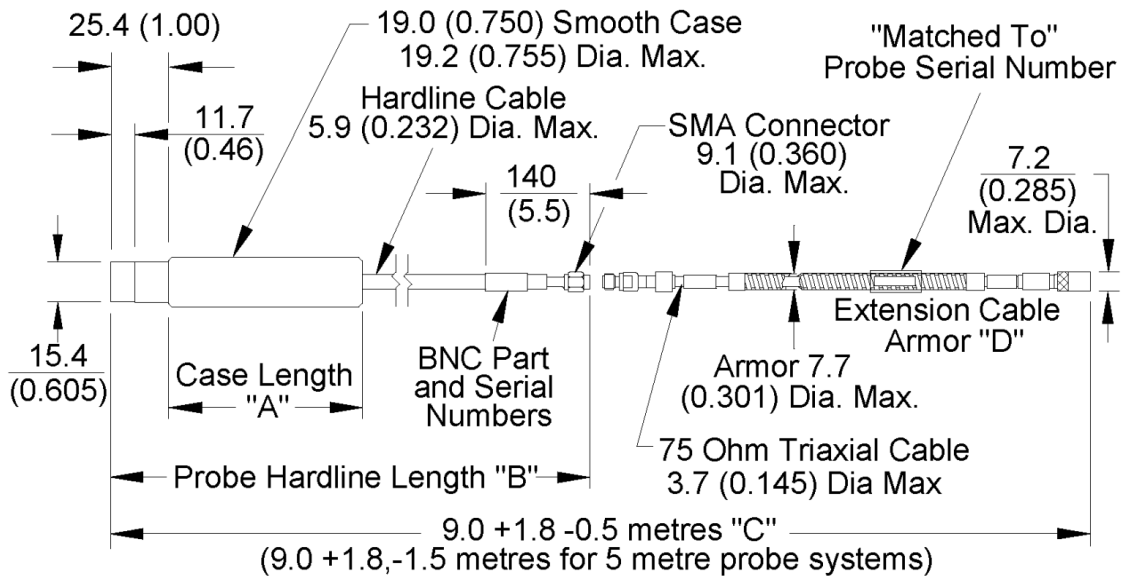
Figure 9: 330303 HTPS Smooth Case Probe
