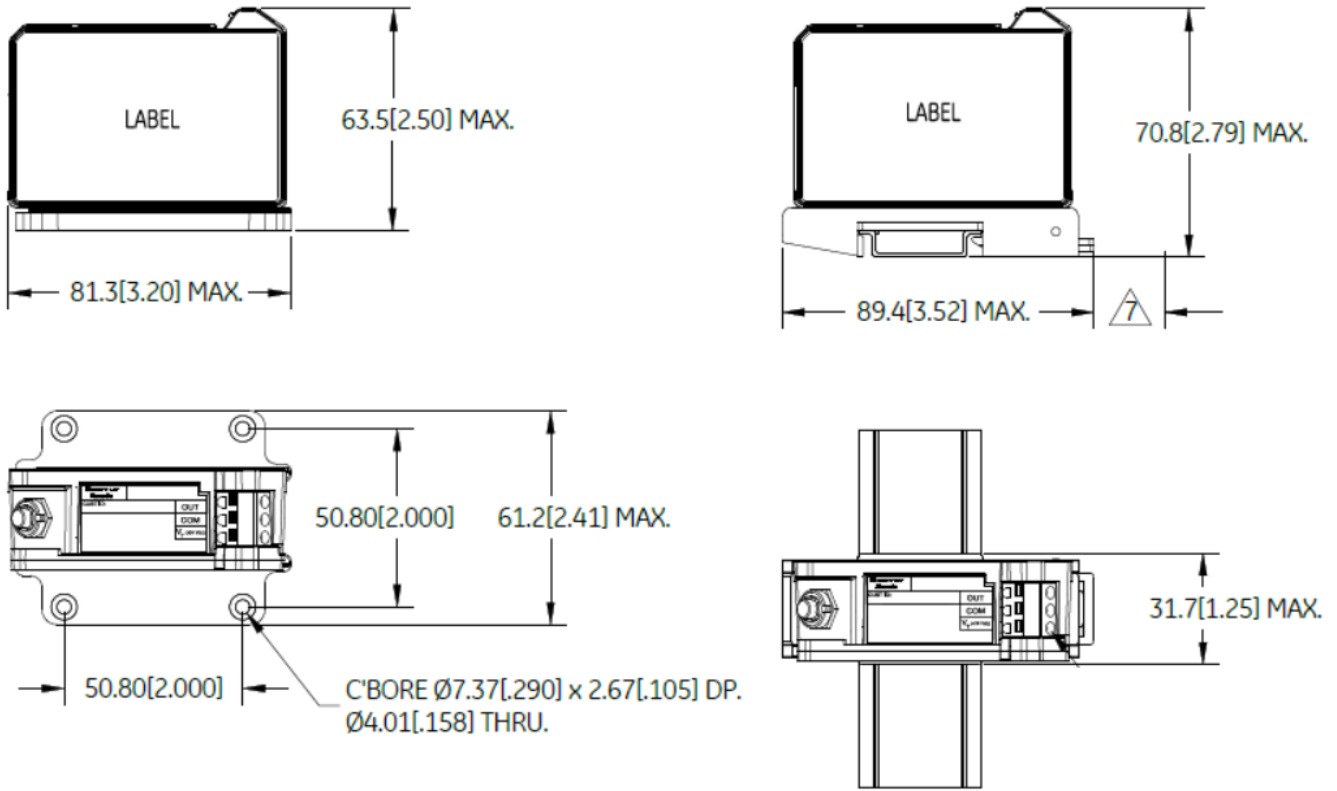
Figure 11: 330380 HTPS Proximito Sensor (see drawing of same number)
