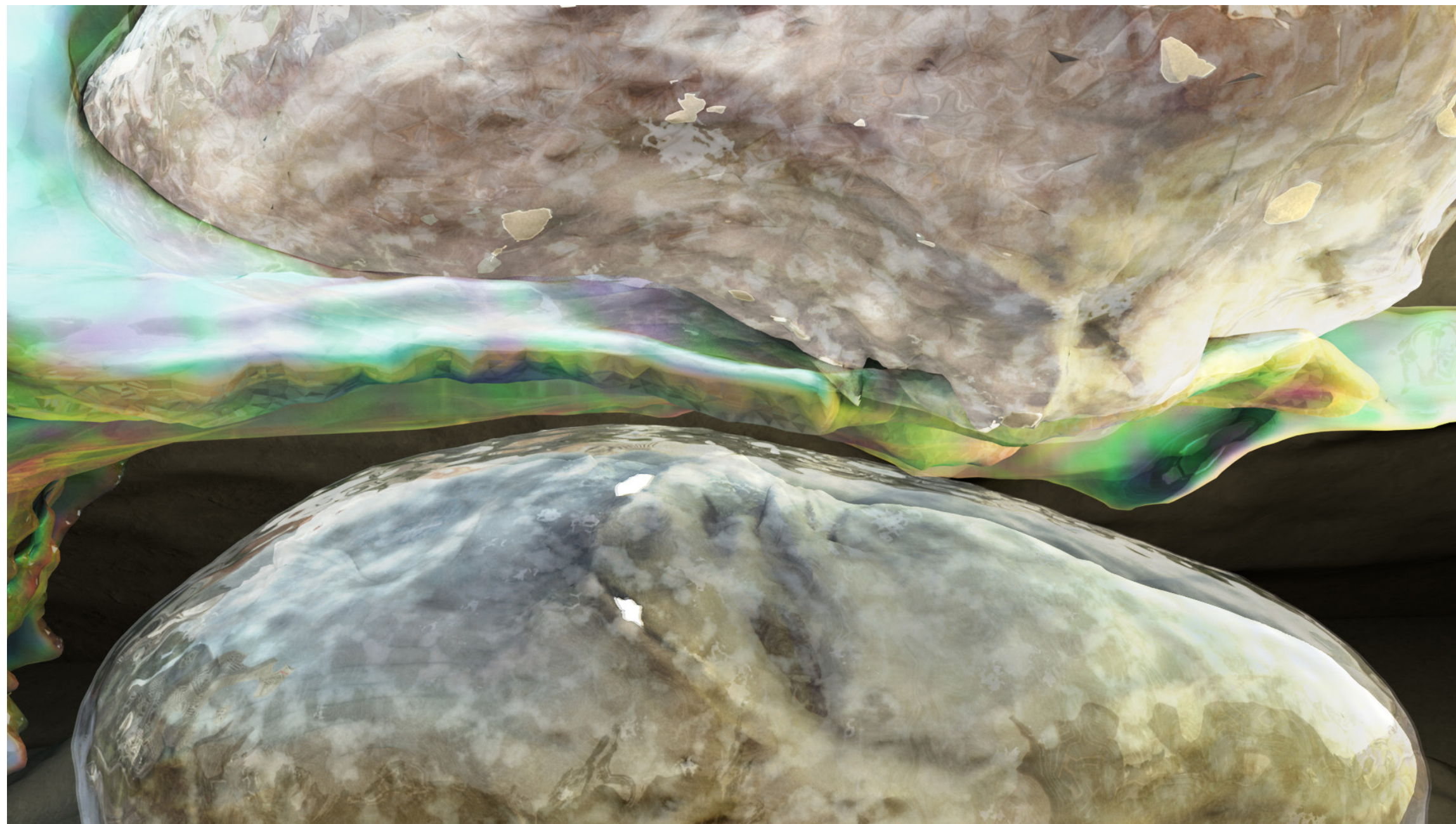
Polymer attaches to the sandstone formation through a covalent bond—preferentially in tight spots (pore throats). The highly water-wetting polymer “lays down” in the presence of hydrocarbons (repelled).
