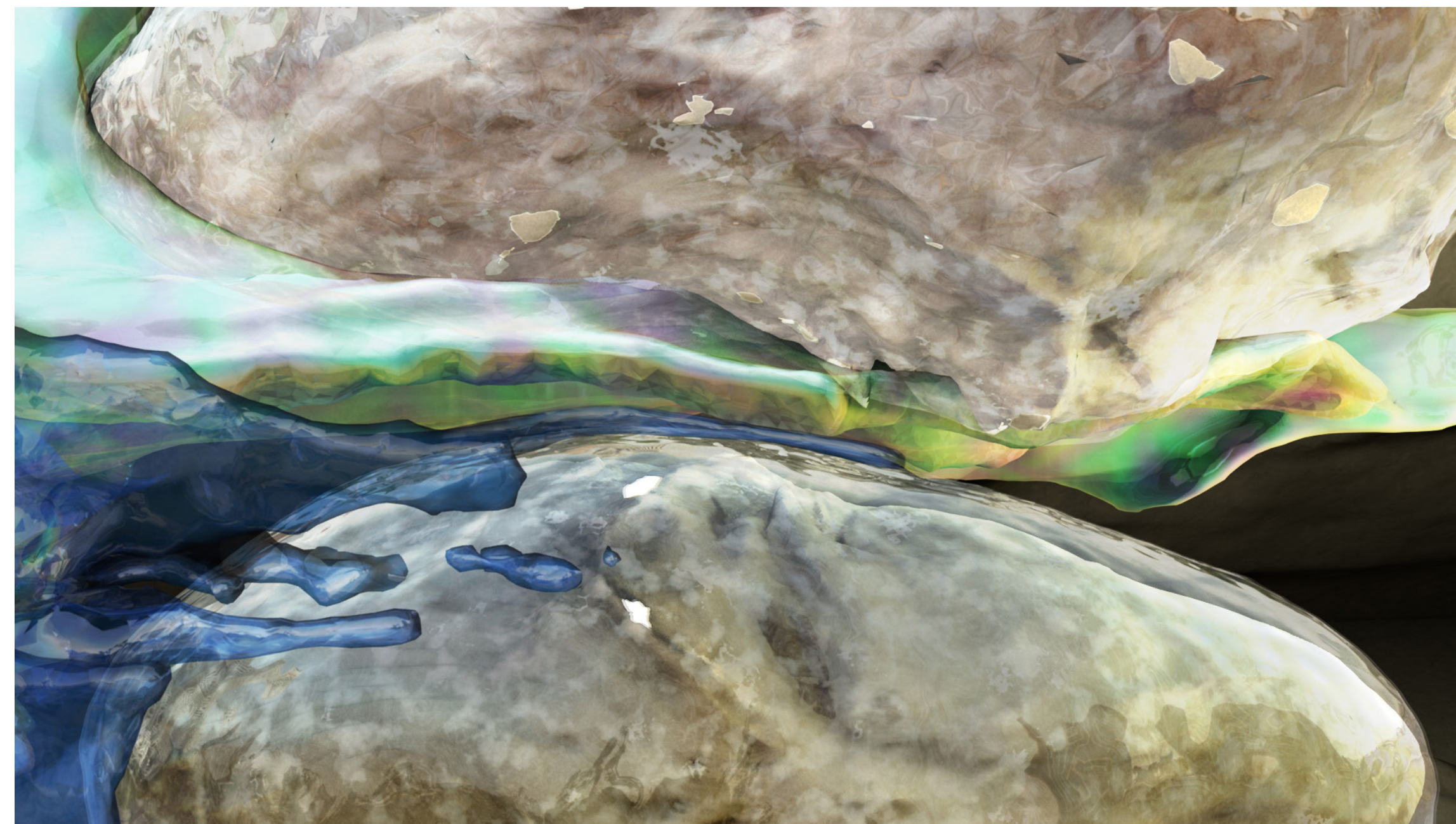
In the presence of water, the highly water-wetting polymer expands, filling pore throats, thereby increasing resistance to water flow ( R_w ).
