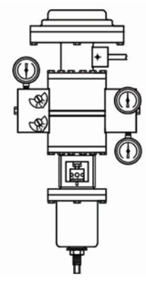
Figure 6.4 - Model HPP-4 Direct-Acting Positioner (Split Range)
