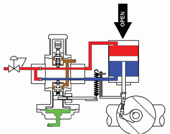
Figure 4.3 - Decrease in Instrument Input Signal to OPEN Valve. A decrease in the instrument input signal causes the internal pistons to move down, simultaneously loading Cylinder Top and unloading Cylinder Bottom. The actuator pressure differential moves the valve toward the OPEN position.
