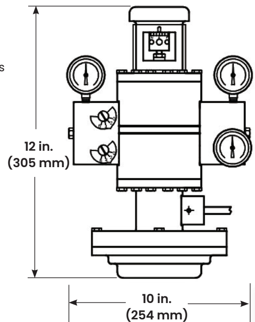
Figure 5 – Overall dimensions of HPP-4 positioner (standard range)
