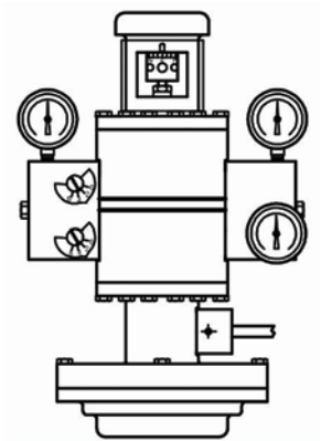
Figure 6.1 - Model HPP-4 Reverse-Acting Positioner (Standard Range)
