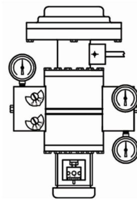
Figure 6.3 - Model HPP-4 Direct-Acting Positioner (Standard Range)
