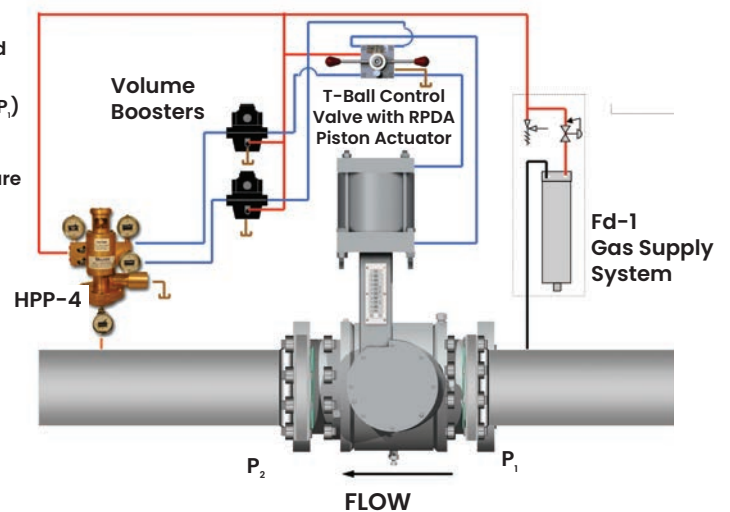
Figure 2 – HPP-4 positioner installed on Becker RPDA Series Actuator. The HPP-4 positioner may be utilized with any of Becker's products' double-acting series actuator for accurate positioning of control valves. The HPP-4 positioner is designed to accept a pneumatic instrument signal from an I/P transducer or a pneumatic controller. The HPP-4 positioner is available in both reverse and direct-acting with a variety of instrument signal input ranges. The configuration shows the HPP-4 positioner mounted on a Becker RPDA actuator with an optional NBV-100 to shutoff bleed when the control valve is at both full-open and full-closed positions. Additionally, the HPP-4 positioner is equipped with VB-250 Series Volume Boosters to provide increased flow capacity for large control valve actuators and/or high speed applications such as power plants.
