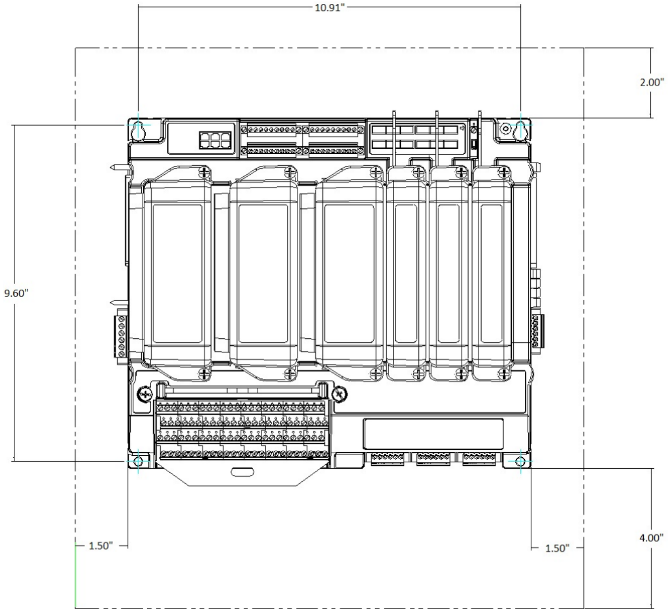
Figure 1: Dimensional Drawing and Enclosure Clearances.
