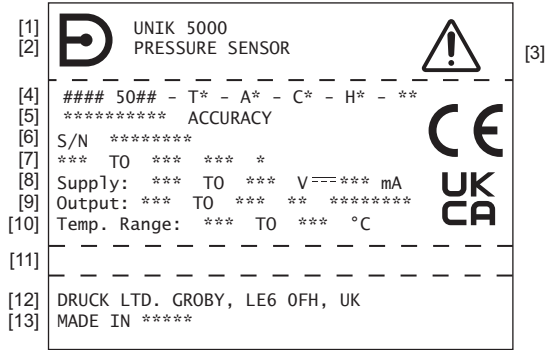
Figure 2: Identification, Electrical and Pressure Markings
